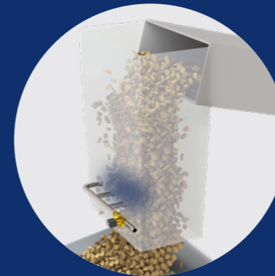
CONVENTIONAL EXTINGUISHING SYSTEM
